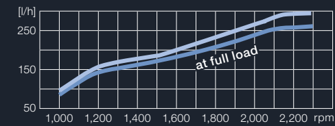
Fuel Consumption V12-1400 / V12-1550
