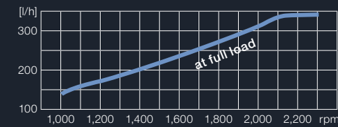
Fuel Consumption V12-1800
